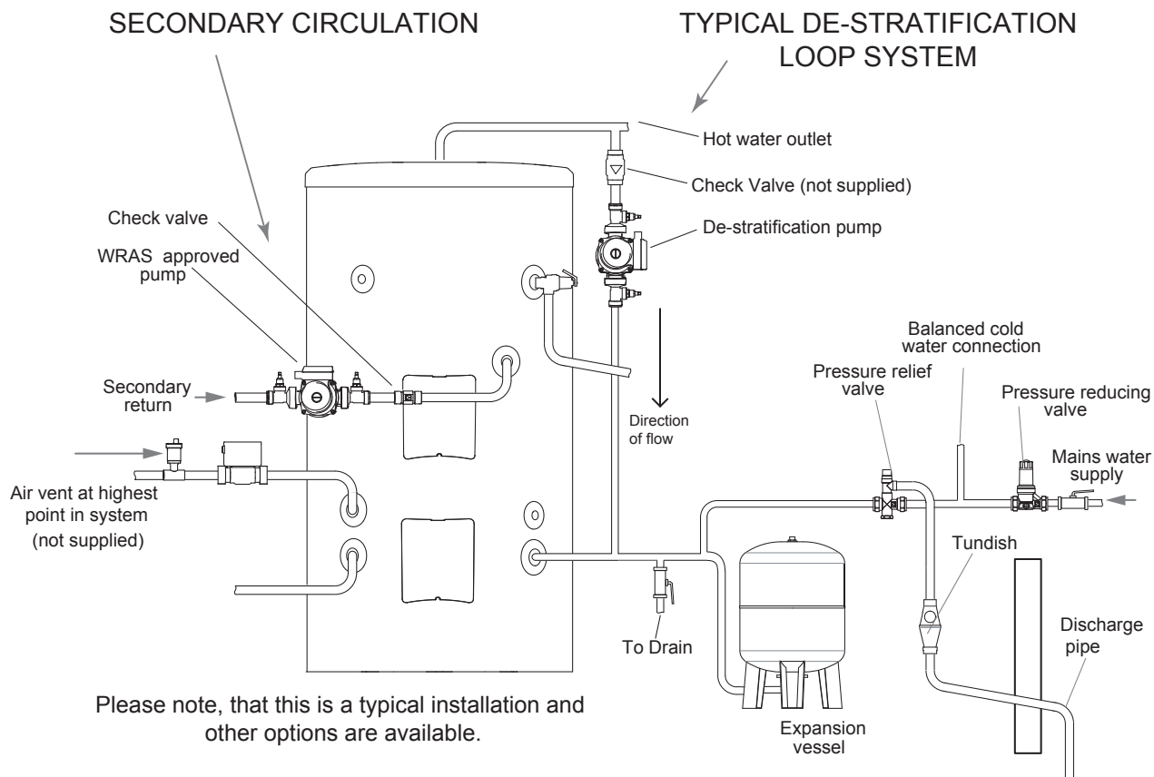
Figure 08: Schematic installation
