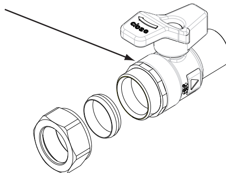
Figure 17 - Exploded View of Isolating valve
