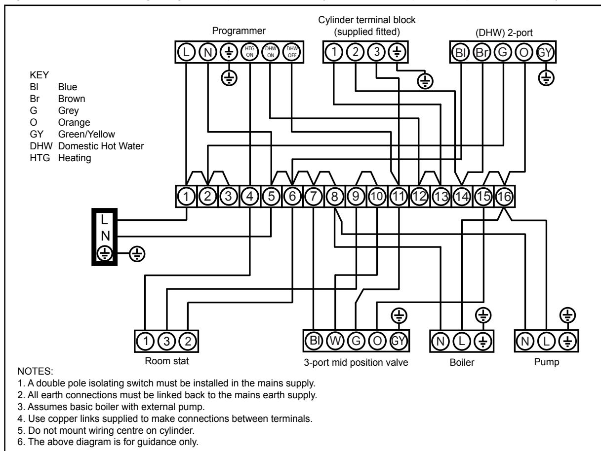
Fig: 06: Schematic Wiring Diagram - 2 port valve in conjunction with 3 port mid position valve system. (Y plan).
