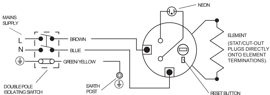
FIGURE 06: WIRING DIAGRAM
