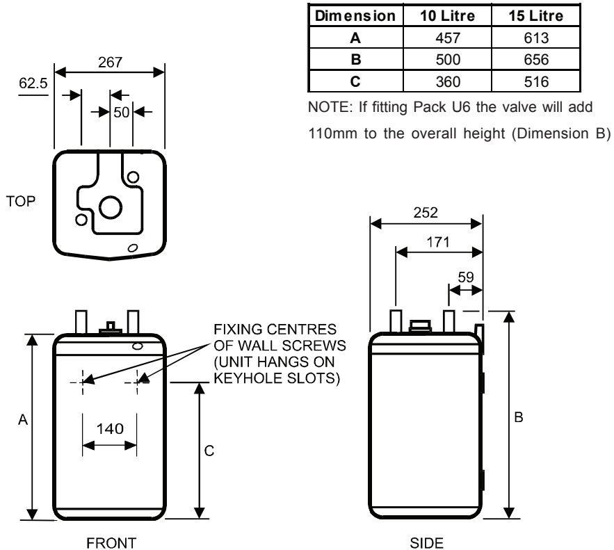
FIGURE 01: DIMENSIONS
